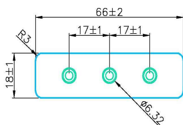
Male Part PT0095 M
