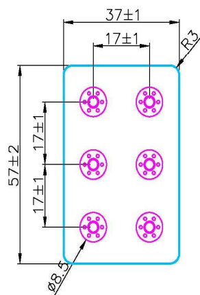
Female Part Art.nr. PT0078 F
